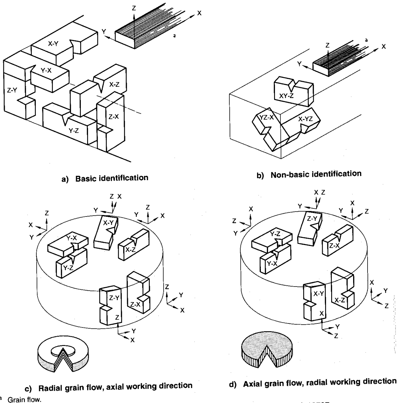
Figure 11 — Fracture plane orientation identification as in ISO 12737
