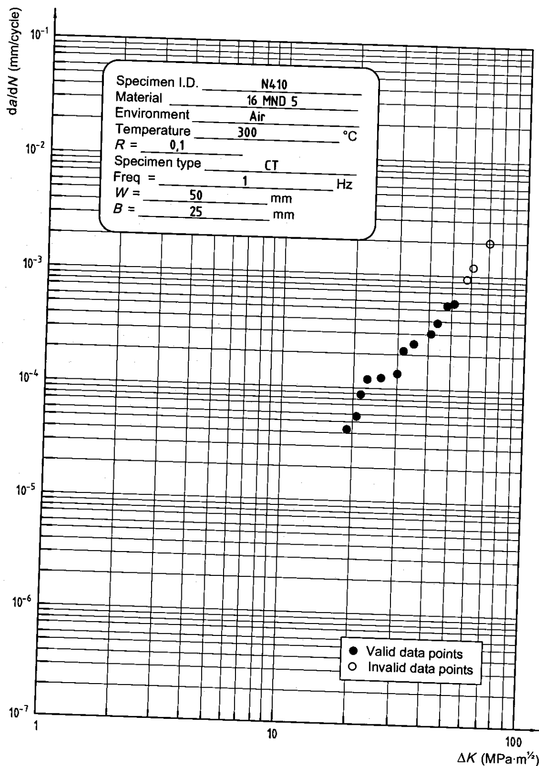
Figure 18 — Example plot of fatigue crack growth test result
