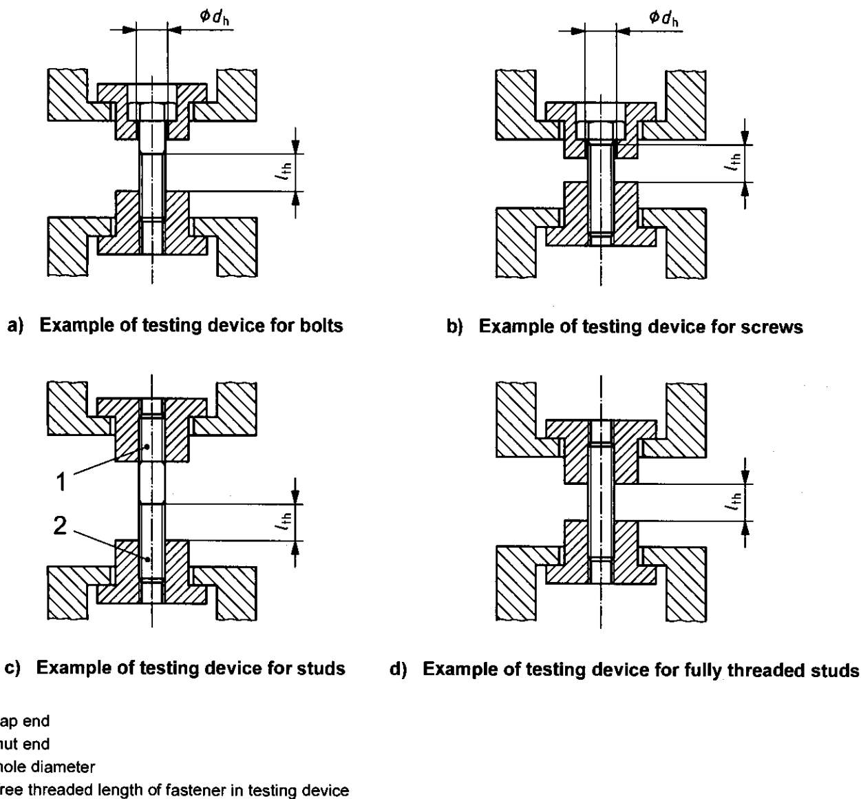
Figure 2 — Examples of testing devices
